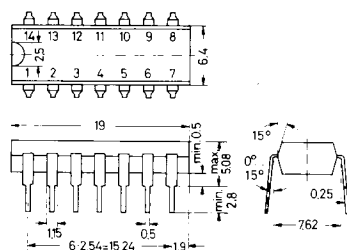
Fig. 3: MDA 2062 in 14-pin Dip Plastic Package TO-116, 20 A 14 according to DIN 41870
