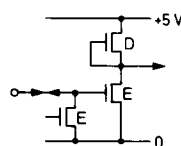
Fig. 7: Pin 10, Input/Output
