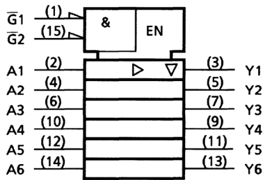
TC74HC365A
