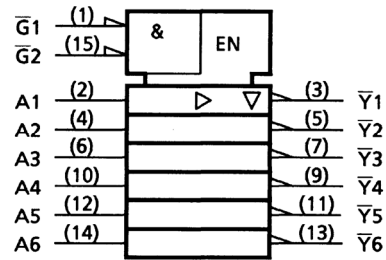
TC74HC366A
