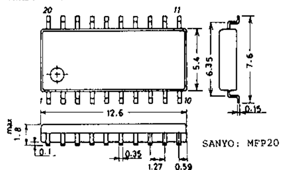
外形図 3036B~3020IC [LC7880M] (unit: mm)
