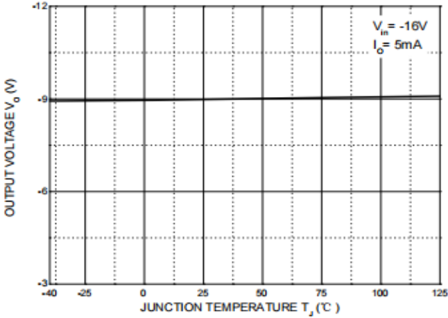
Fig 5: Output Voltage vs Junction Temperature
