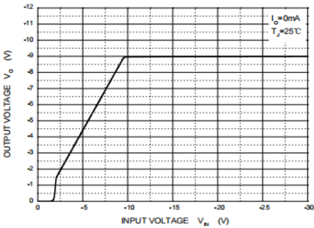
Fig 1: Output Characteristics
