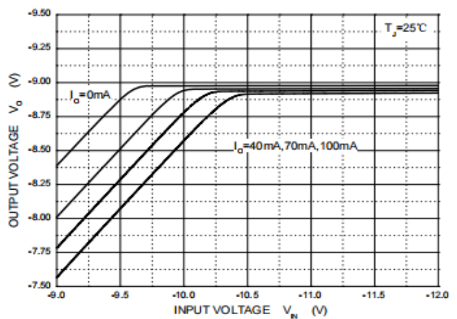
Fig 3: Dropout Characteristics
