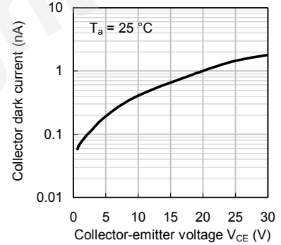
Collector Dark Current vs. Collector-Emitter Voltage
