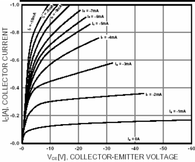
Fig.3 Static Characteristic
