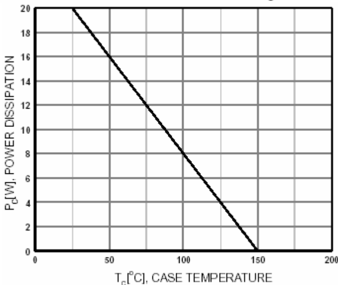
Fig.7 Power Derating
