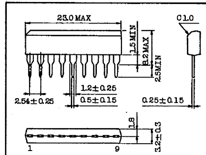
JEDEC — TOSHIBA S9A-P OUTLINE(1)
