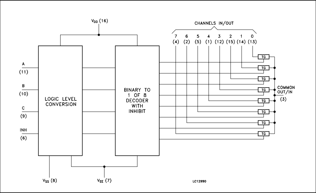
Figure 5. Functional diagram
