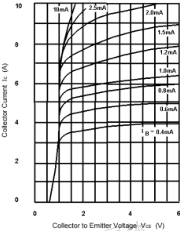
Fig.3 Static Characteristic
