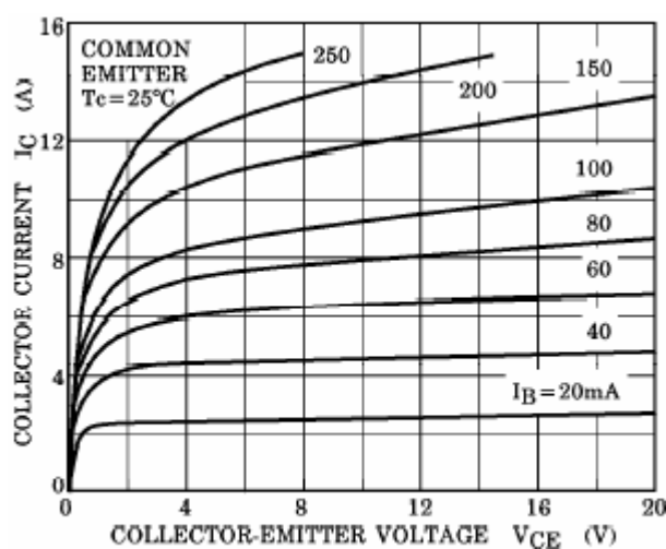
Fig.3 Static Characteristic
