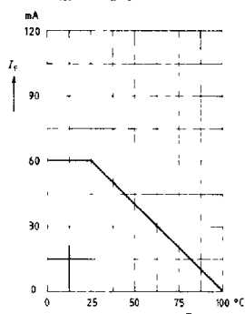
Permissible loss diode P_{tot} = f(T_{amb})
