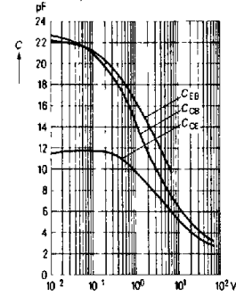
Transistor capacitances C = f(V_{CE}) ( T_{amb} = 25^\circ\text{C} , f = 1 \text{ MHz} )
