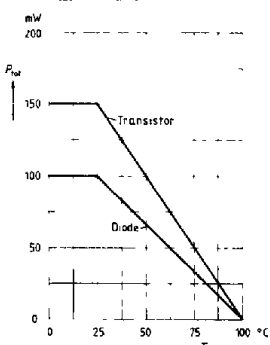
Permissible loss transistor P_{tot} = f(T_{amb})
