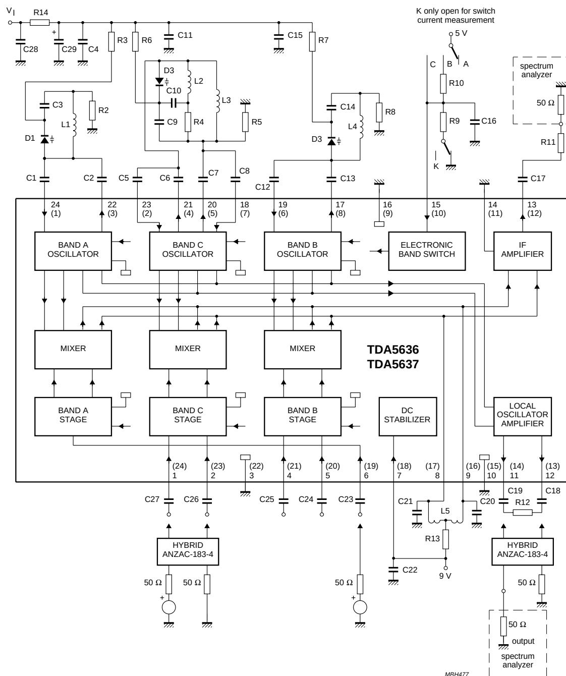
Fig.17 Measurement circuit.
