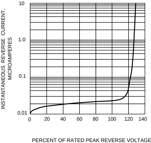
FIG.4-TYPICAL REVERSE CHARACTERISTICS
