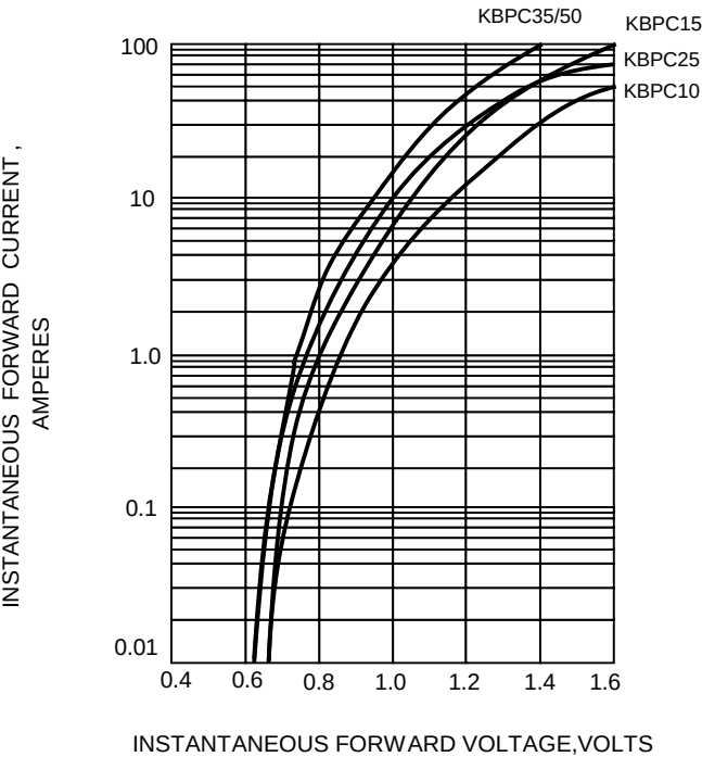
FIG.3-TYPICAL FORWARD CHARACTERISTICS
