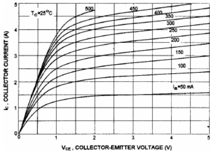
Fig.3 Static Characteristic
