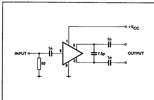
Fig. 2 Test circuit
