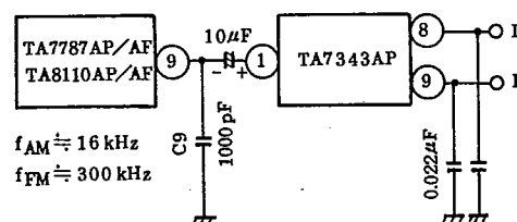
Fig.5 CONNECTION TO TA7343AP
