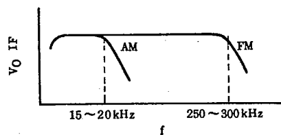
Fig.6 FREQUENCY CHARACTERISTICS OF DET OUTPUTS
