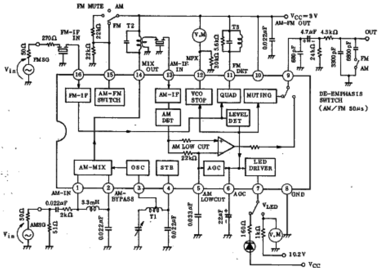
TEST CIRCUIT 1
