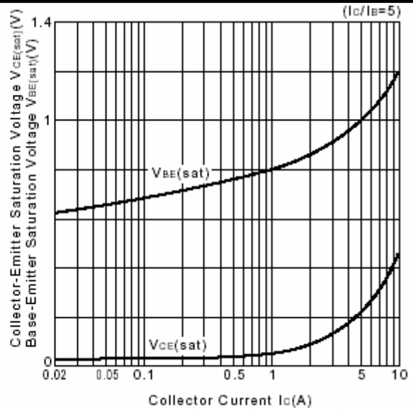
Fig.4 Base-Emmitter Saturation Voltage Collector-Emmitter Saturation Voltage
