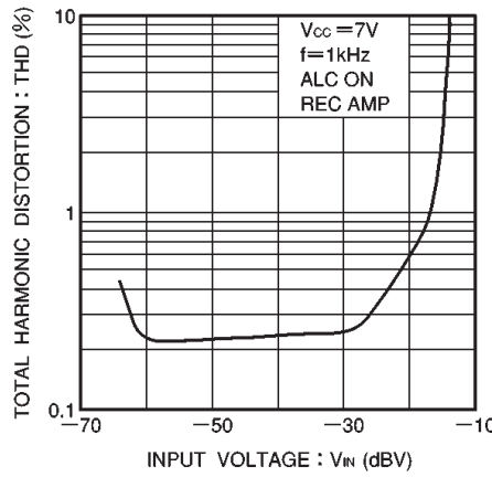
Fig. 9 Total harmonic distortion vs. input voltage
