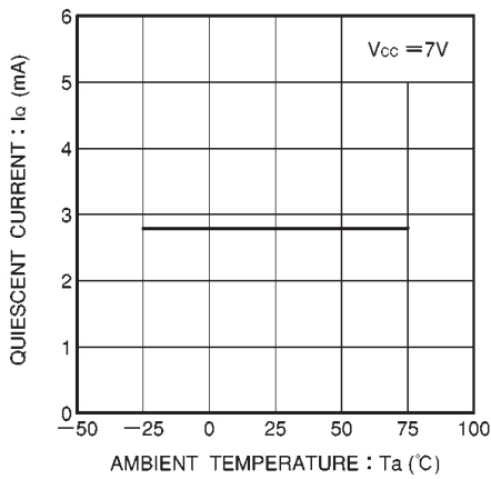
Fig. 11 Quiescent current vs. ambient temperature
