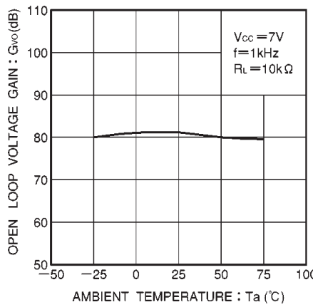
Fig. 12 Open loop voltage gain vs. ambient temperature
