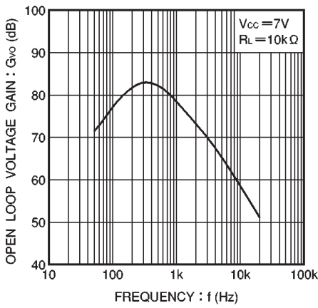
Fig. 8 Open loop voltage gain vs. signal frequency
