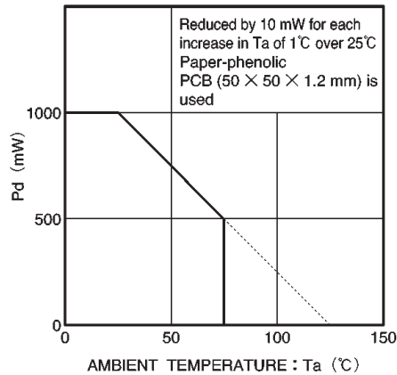
Fig.4 Power dissipation curve (BA6246N, BA6247N)
