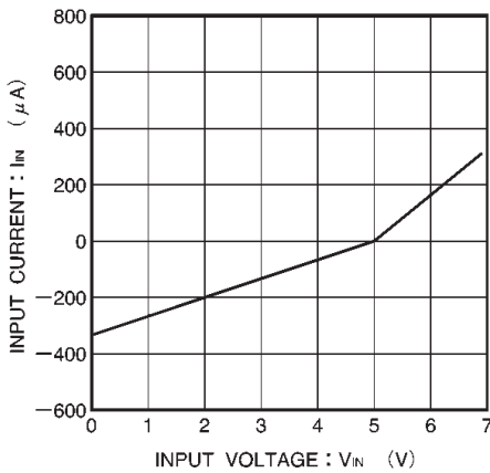
Fig.6 Input voltage vs. input current (BA6246N)
