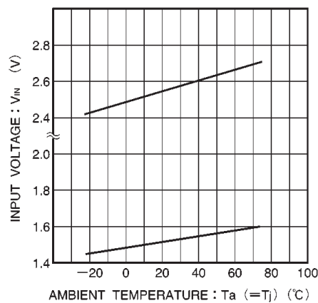
Fig.8 Input voltage vs. ambient temperature
