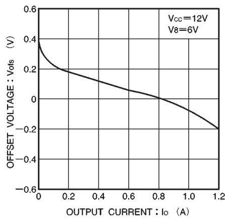
Fig.11 Offset voltage vs. output current
