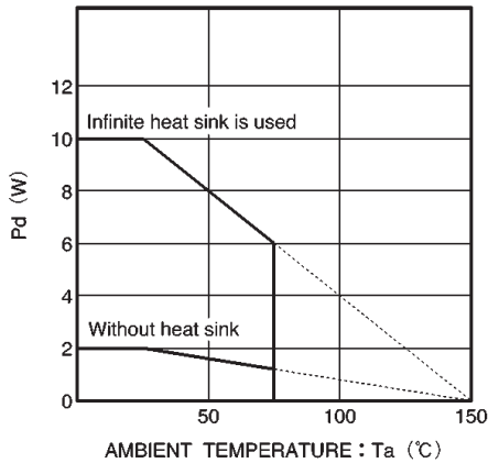
Fig.3 Power dissipation curve (BA6247)
