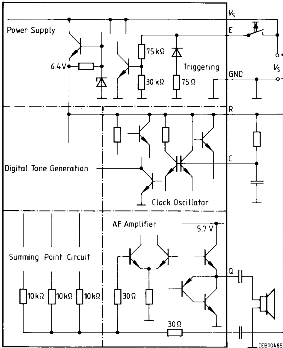
Figure 1 Block Diagram
