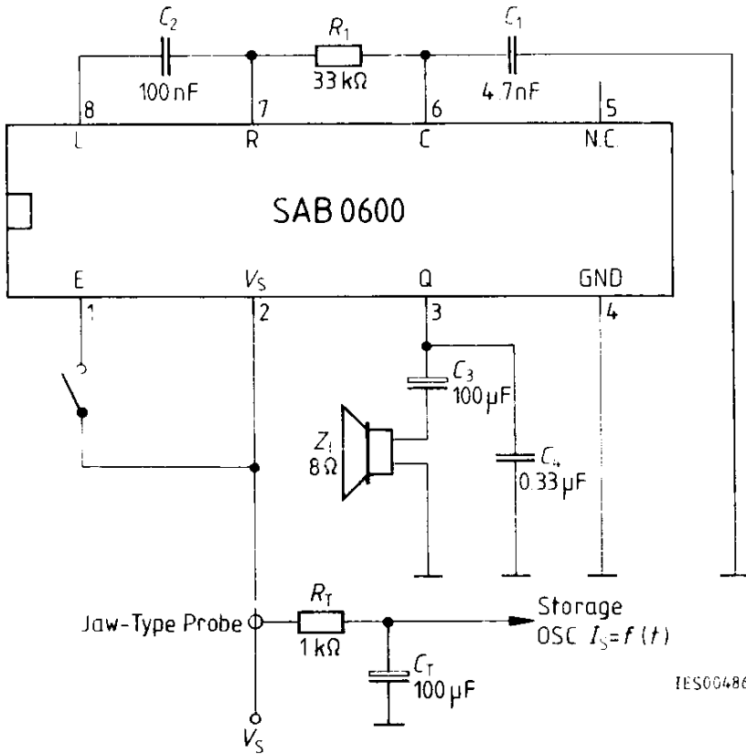
Figure 2 Test Circuit
