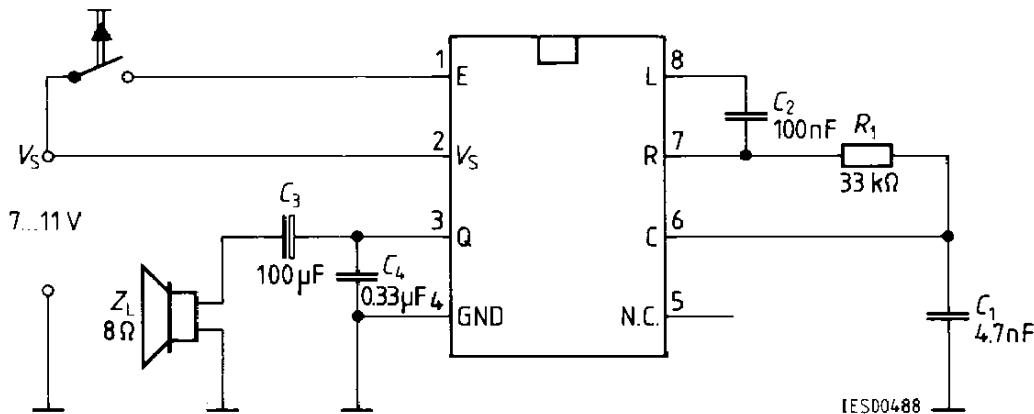
Figure 4 Typical Application Circuit
