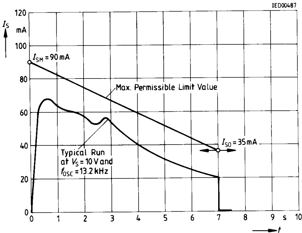
Figure 3 Integral Current Consumption in the Measurement Circuit
