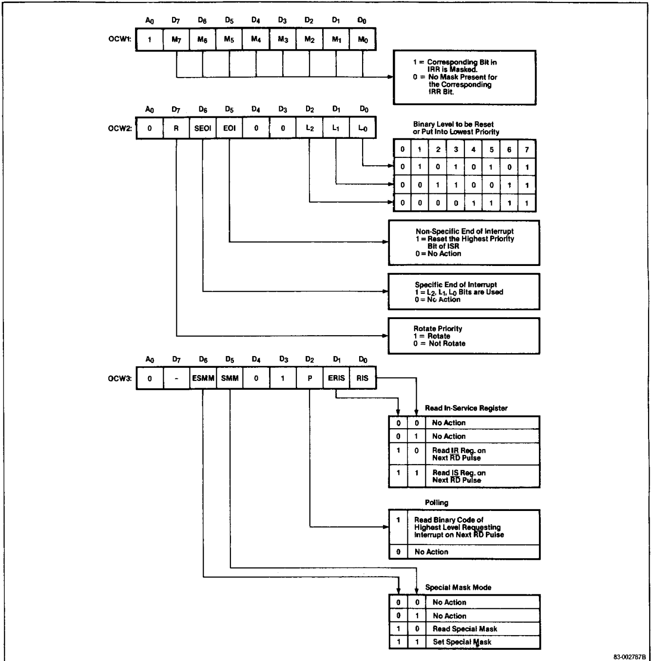
Figure 3. Operation Command Word Format
