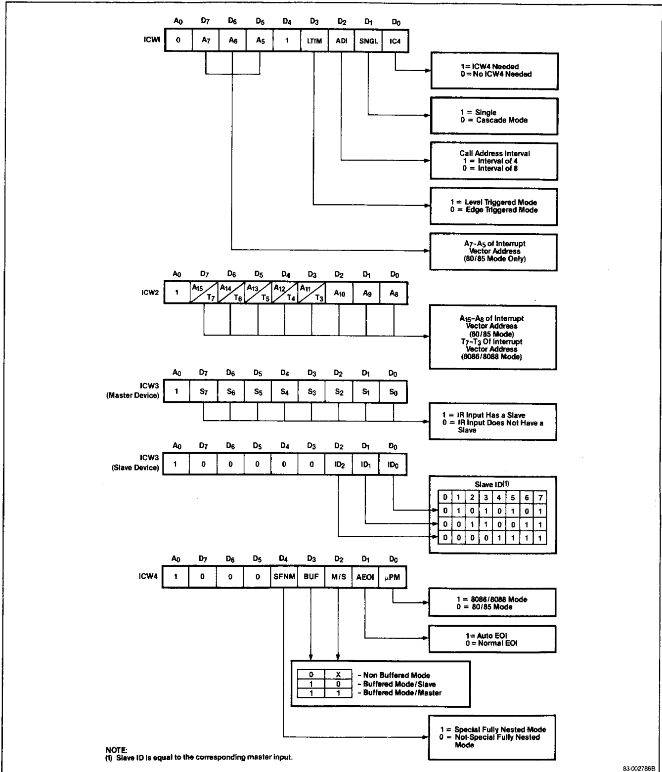
Figure 2. Initialization Command Word Format
