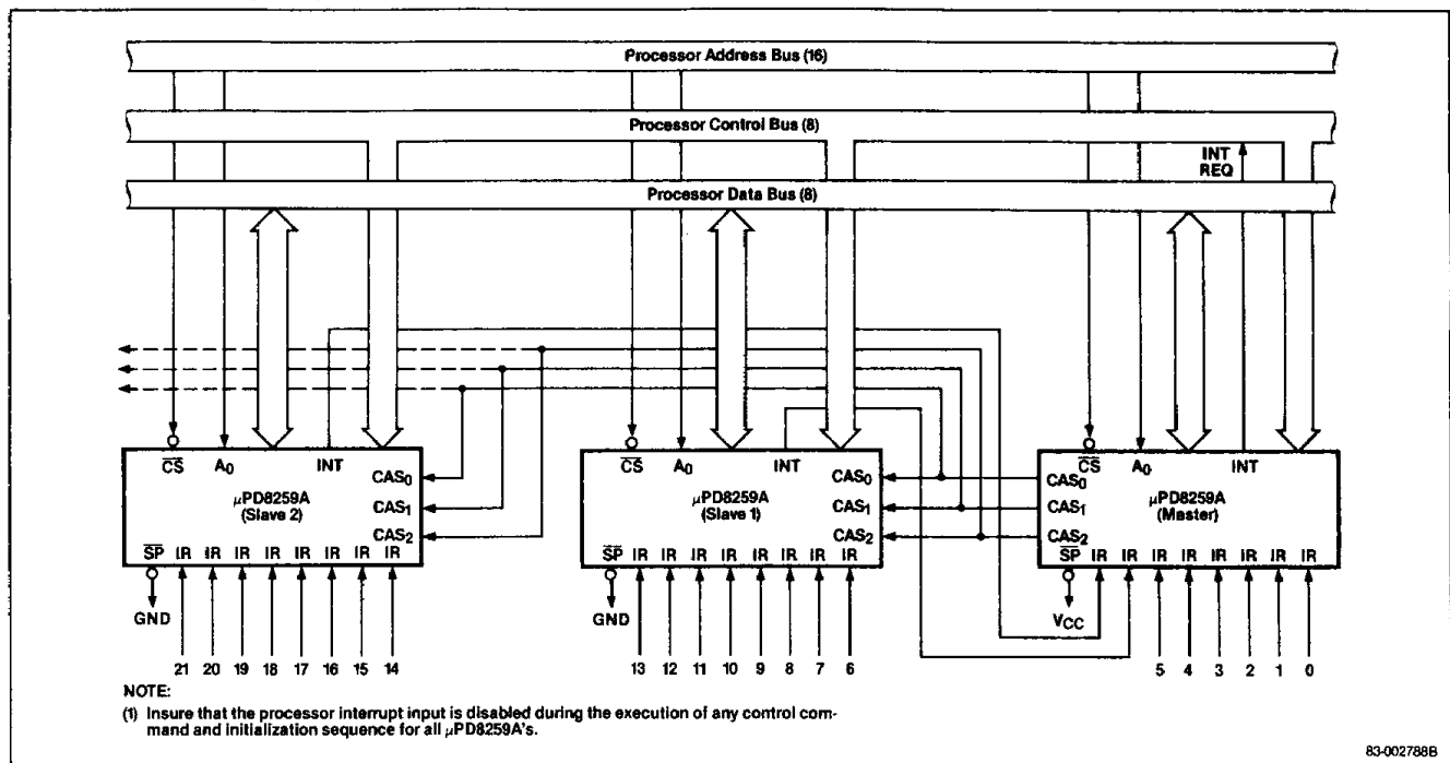
Figure 4. Cascading the μPD8259A
