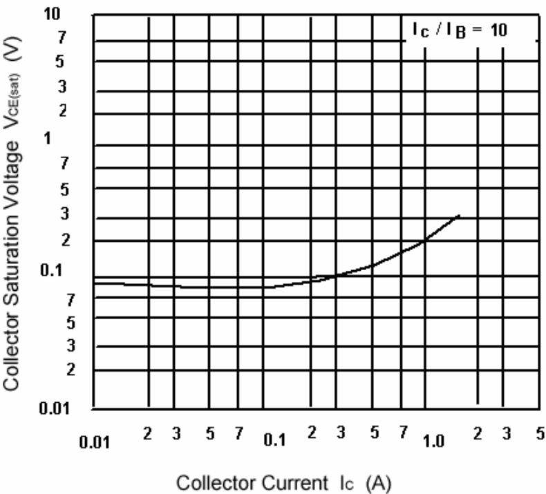
Fig.5 Collector-Emitter Saturation Voltage
