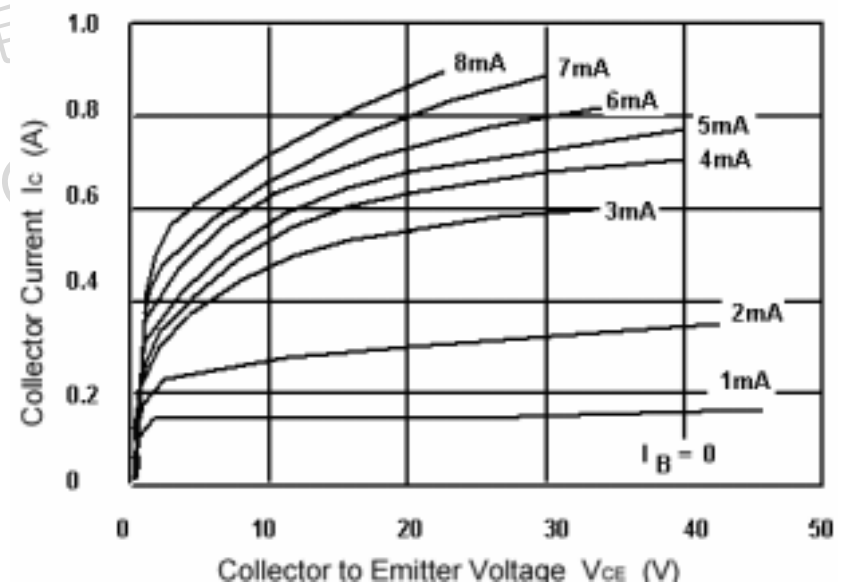
Fig.4 Static Characteristic
