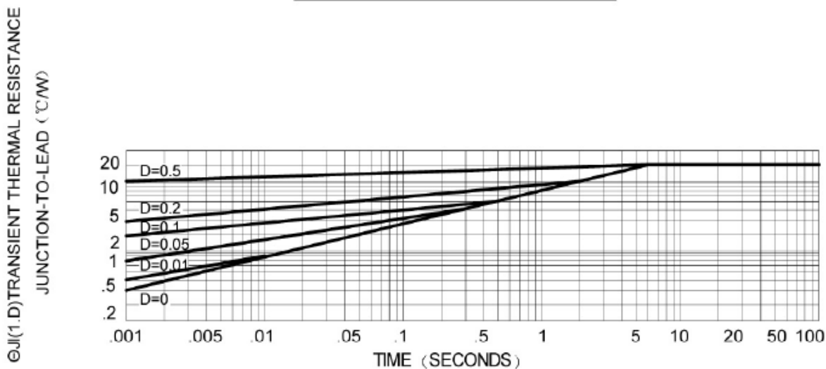
FIG.5 – TYPICAL THERMAL RESPONSE
