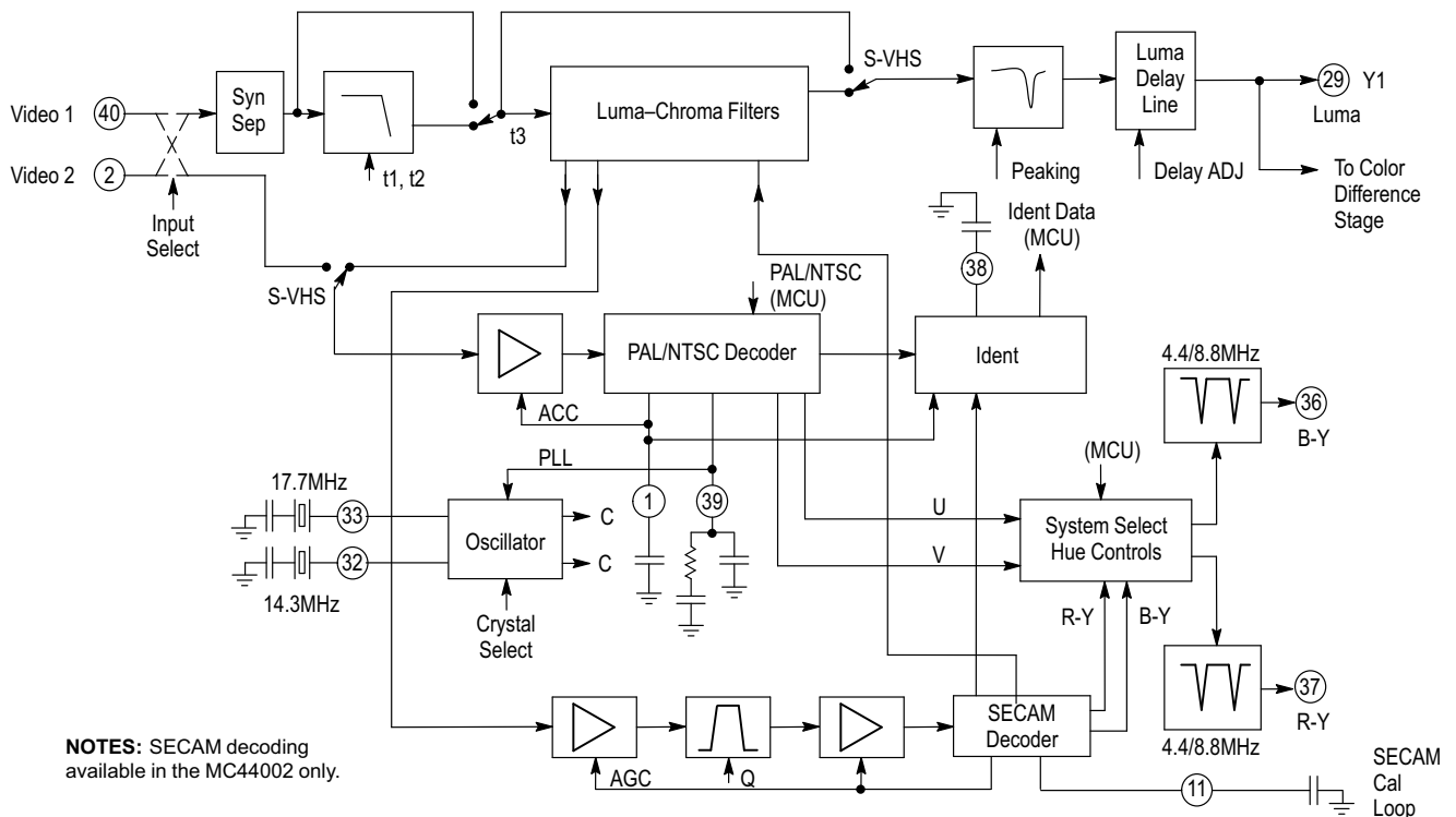
Figure 8. Chroma Decoder
