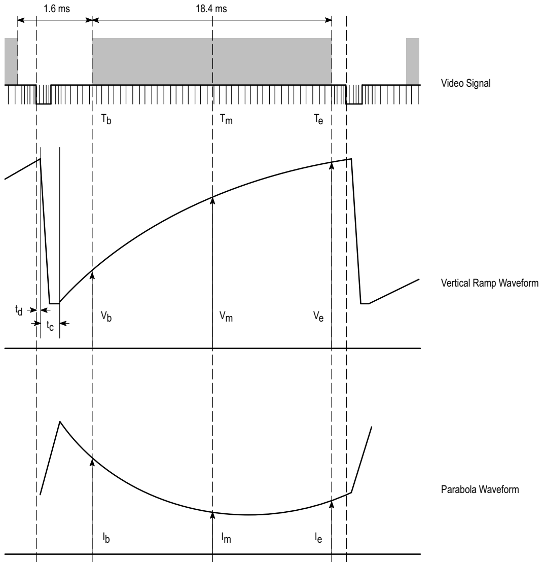
Figure 2. Vertical Waveforms
