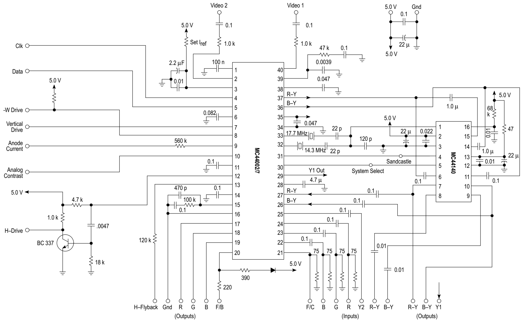
Figure 17. Typical Application Circuit
