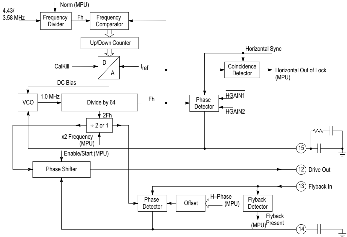
Figure 14. Horizontal Timebase
