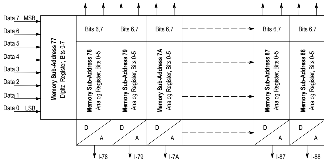
Figure 7. MC44002/7 Memory Map
