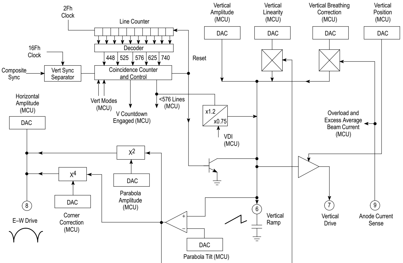
Figure 15. Vertical Timebase
