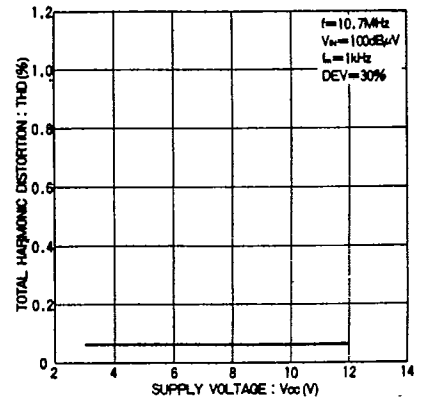
Fig. 18 FM total harmonic distortion vs. supply voltage
