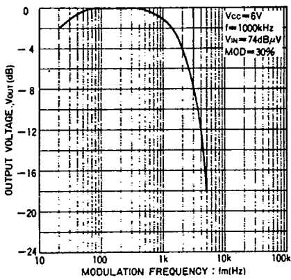
Fig. 34 AM detector output voltage vs. modulation frequency
