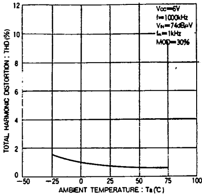
Fig. 31 AM total harmonic distortion vs. ambient temperature
