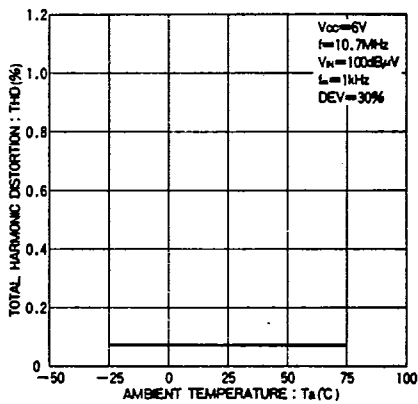
Fig. 19 FM total harmonic distortion vs. ambient temperature
