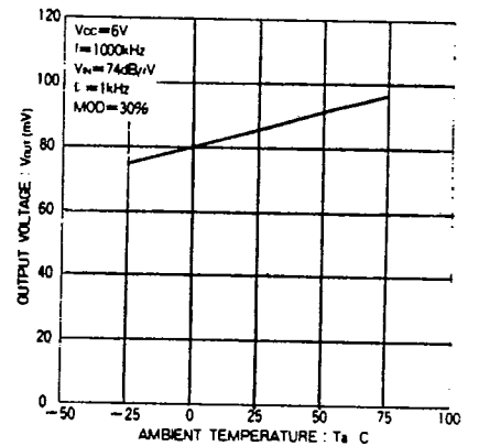
Fig. 27 AM detector output voltage vs. ambient temperature
