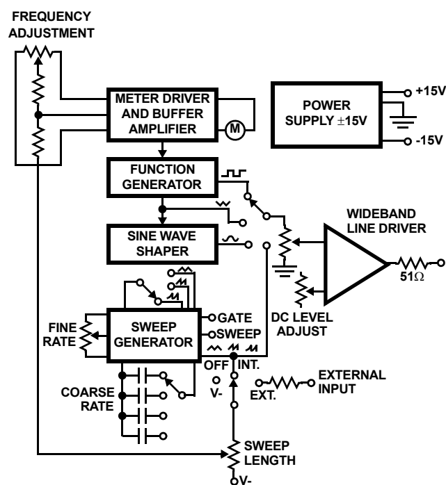
FIGURE 10D. INTERCONNECTIONS
