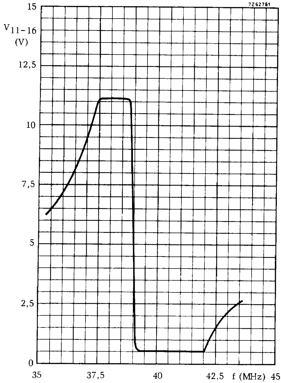
A.F.C. output voltage versus frequency
