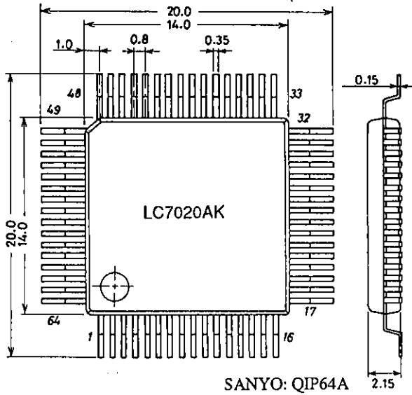
Package Dimensions (unit: mm)
