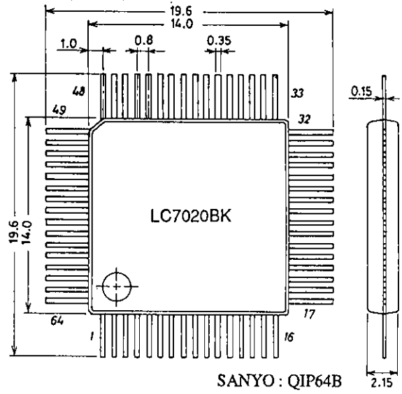
Package Dimensions (unit: mm)
