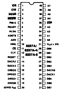
Figure 2. Pin Configuration
