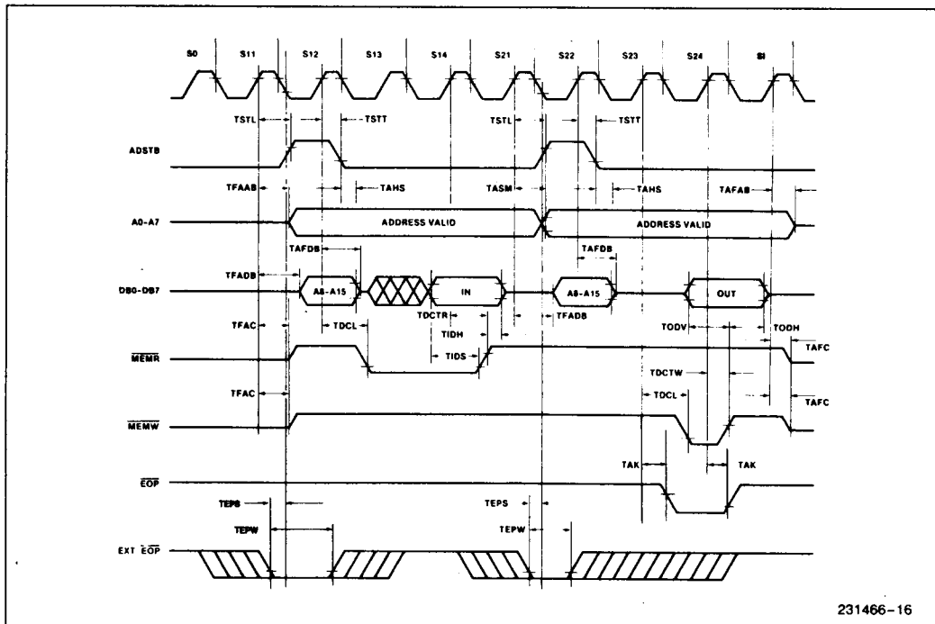
Figure 12. Memory-to-Memory Transfer
