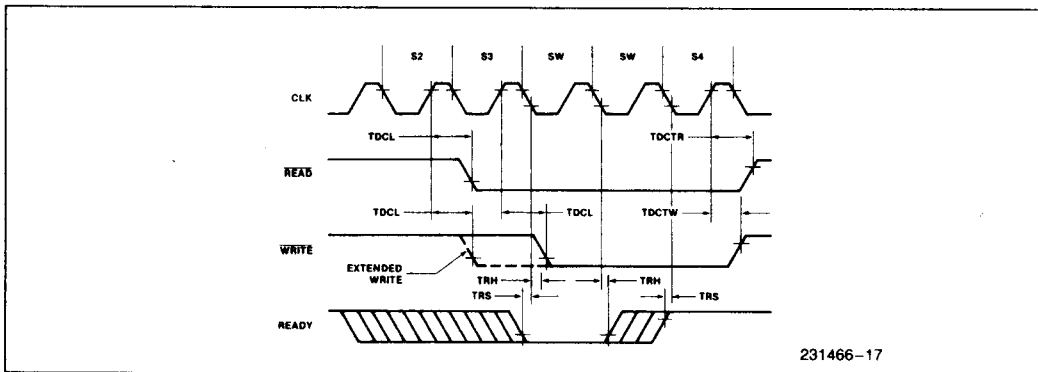
Figure 13. Ready
