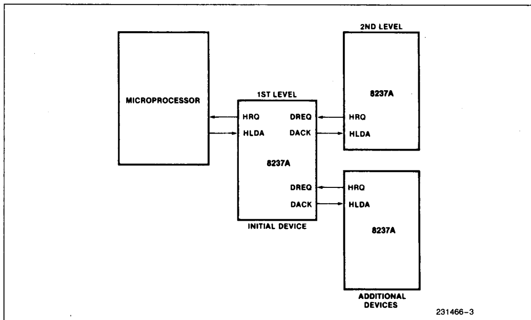
Figure 4. Cascaded 8237As
