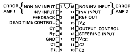
TL495C . . . N PACKAGE
