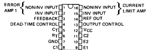
TL494I, TL494C . . . D, J, OR N PACKAGE
