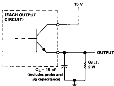
TEST CIRCUIT
