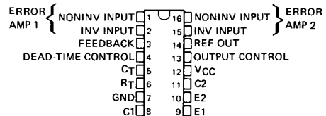
TL495C . . . N PACKAGE
