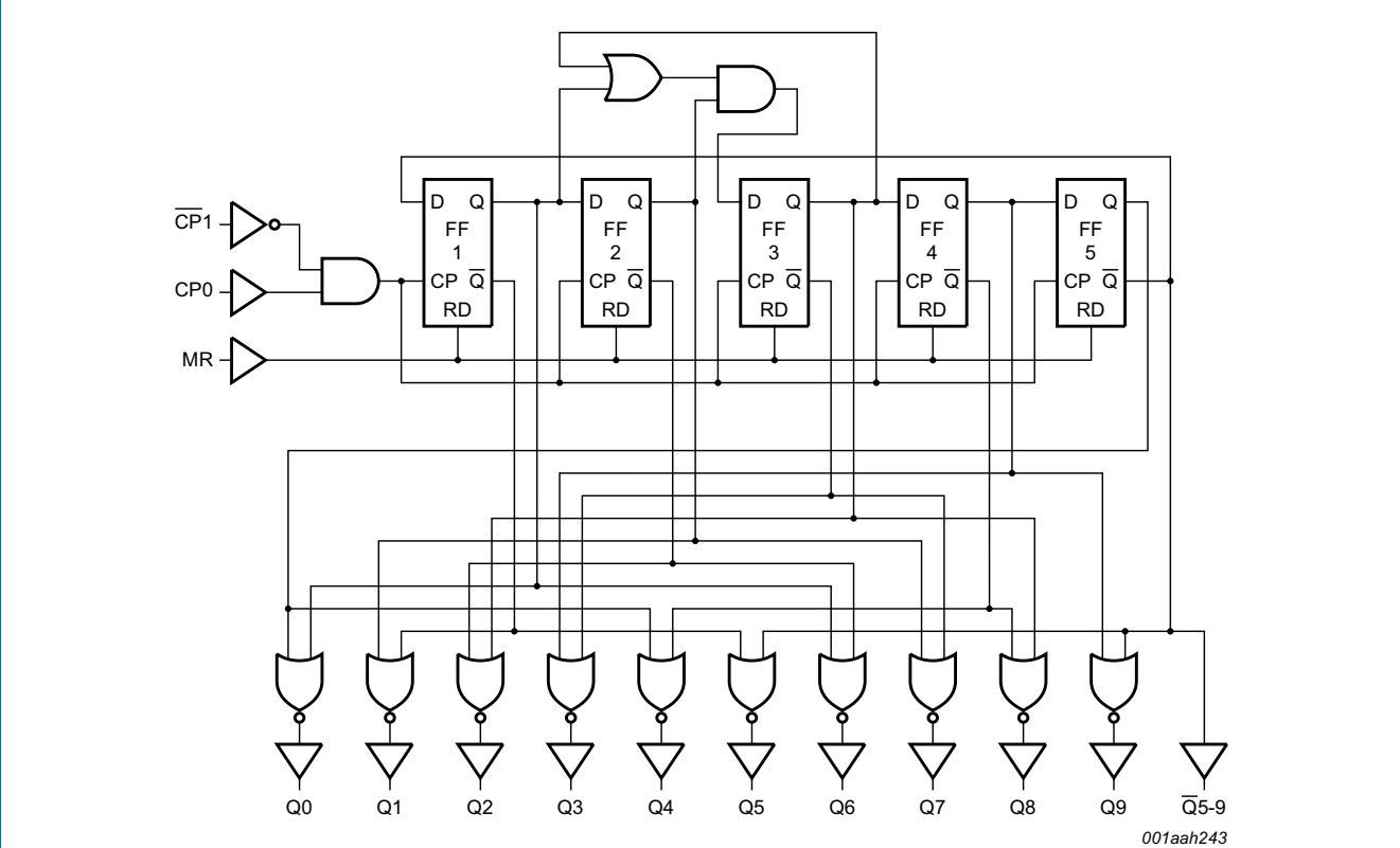
Fig 2. Logic diagram
