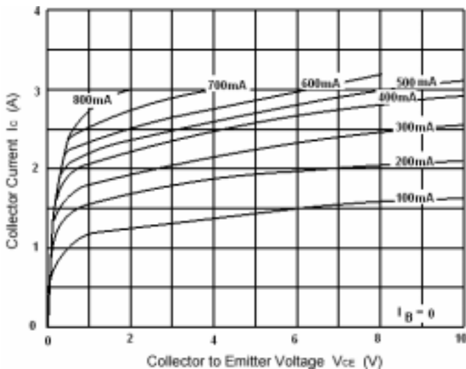
Fig.7 Static Characteristic
