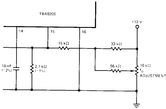
Frequency adjustment range. Test circuit for TBA920S.
