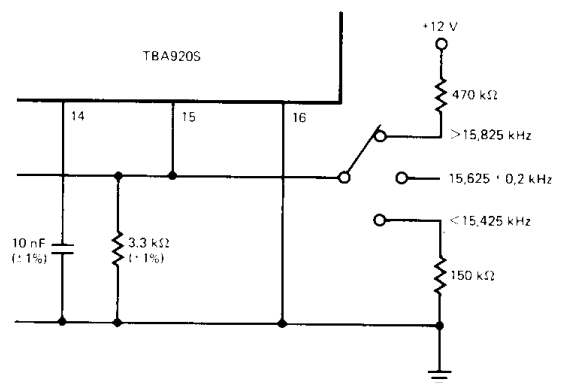
Other circuit possibilities for oscillator frequency adjustment.
