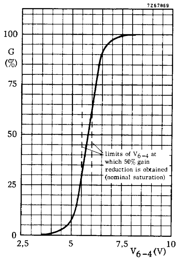
Saturation control of chrominance amplifier
