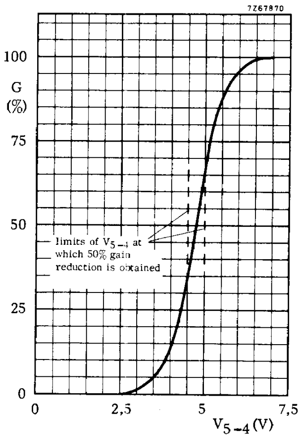
Contrast control of luminance amplifier
