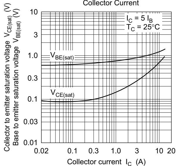
Saturation Voltage vs. Collector Current
