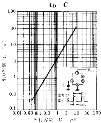
t_0, t_{(ON)} - C_{osc} (AN6249)
