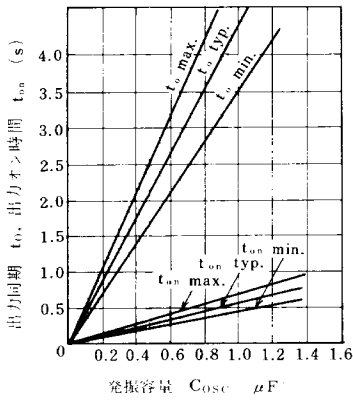
t_0, t_{(ON)} - C_{osc} (AN6249)
