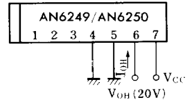
Test Circuit 3 (I OH )
