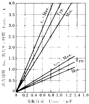
t_0, t_{(ON)} - C_{osc} (AN6250)
