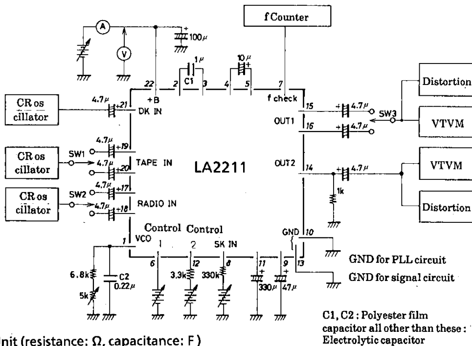
Fig. 1 Test Circuit
