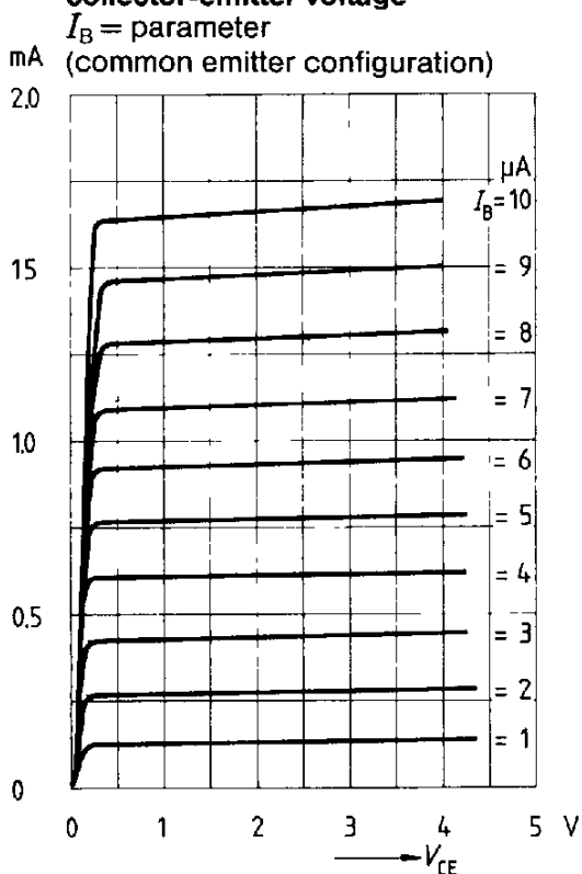
Output characteristics Collector current versus collector-emitter voltage
