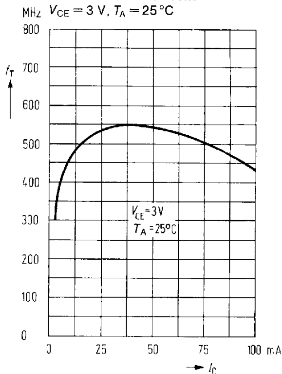
Transition frequency versus collector current V_{CE} = 3\text{ V}, T_A = 25^\circ\text{C}
