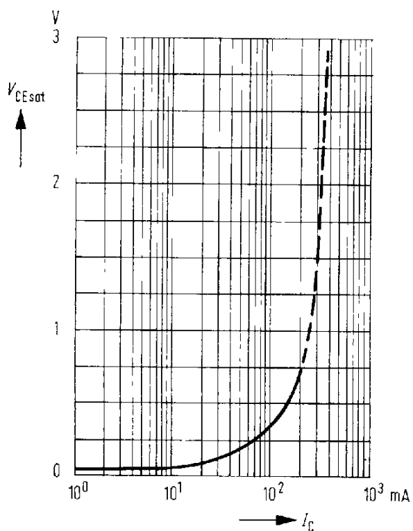
Collector-emitter saturation voltage versus collector current B = 20
