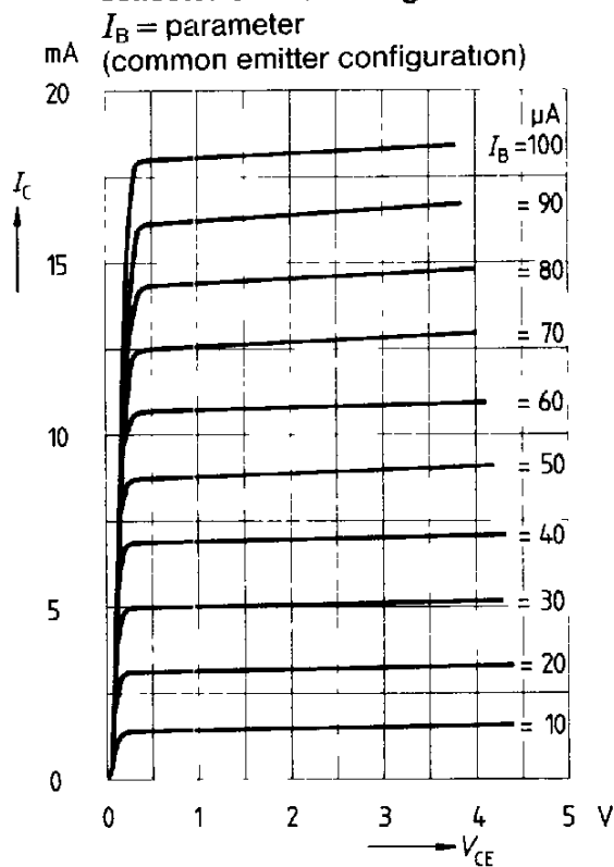
Output characteristics Collector current versus collector-emitter voltage
