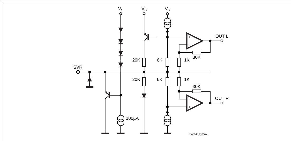
Figure 16. PIN: SVR
