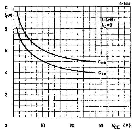
Output and Reverse Capacitance.
