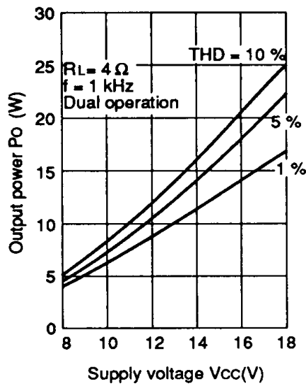
Output power vs. supply voltage (1)
