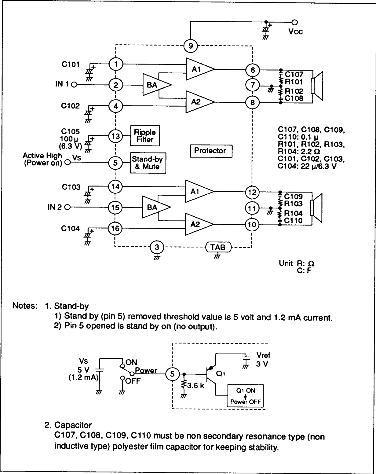
Figure 1 Block Diagram
