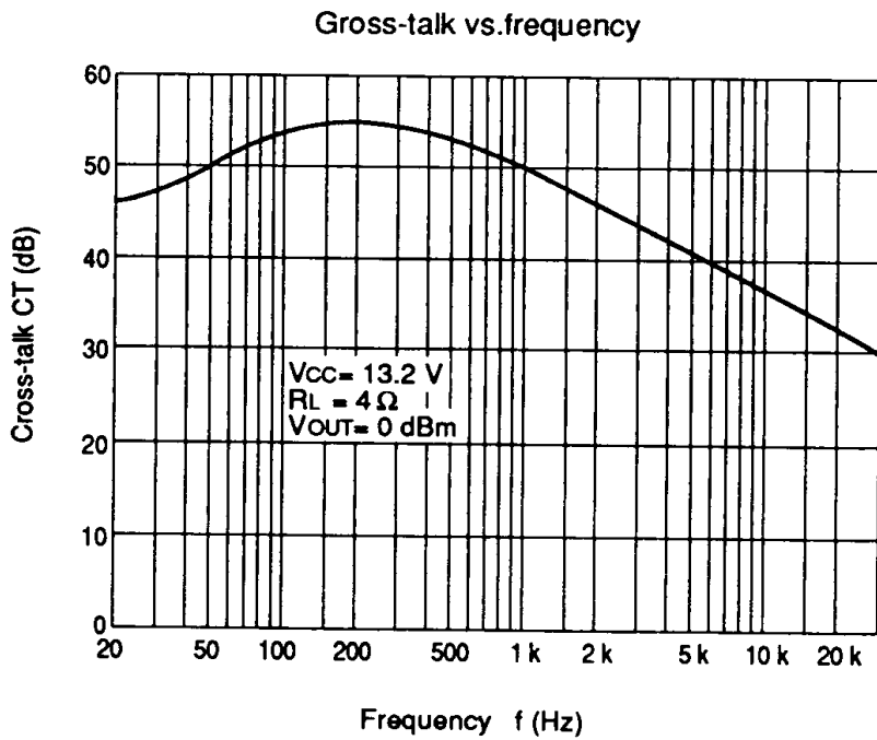
Figure 3 HA13127 Characteristic Curves (cont)
