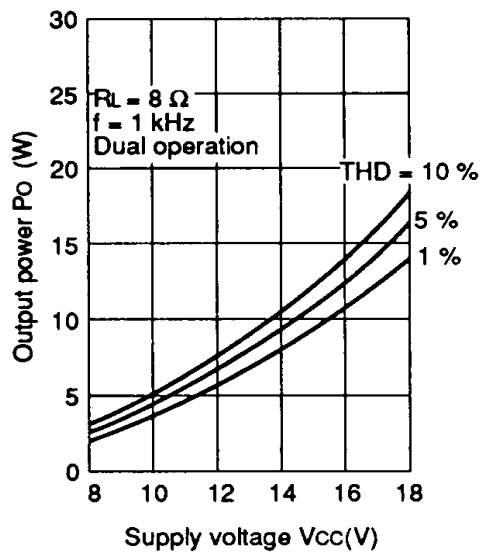
Output power vs. supply voltage (2)
