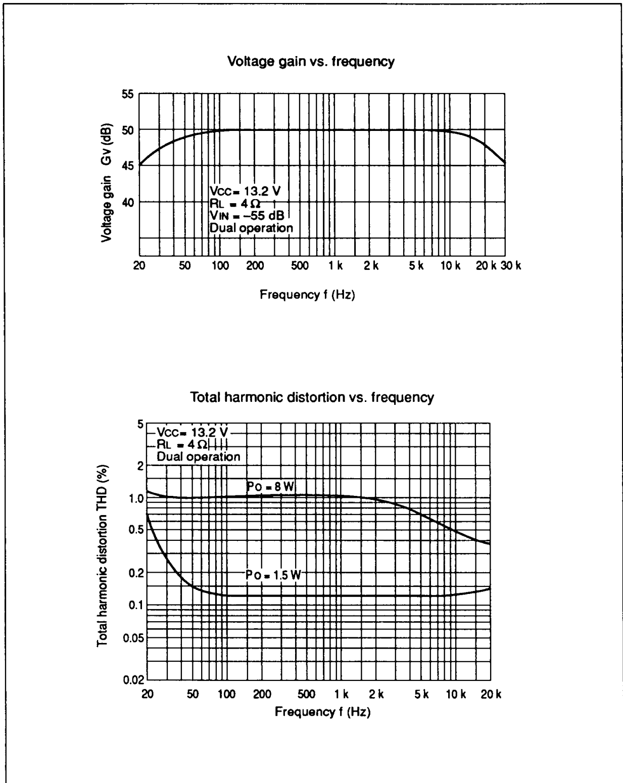
Figure 3 HA13127 Characteristic Curves (cont)
