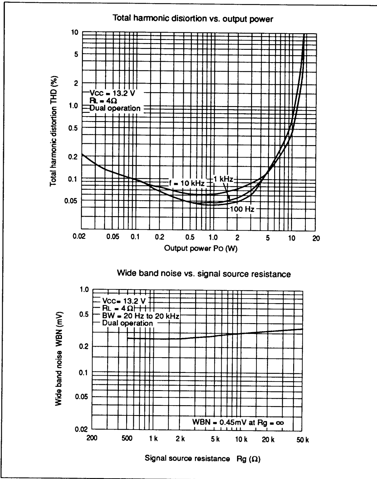
Figure 2 HA13130 Characteristic Curves (cont)
