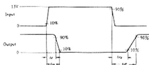
RESPONSE WAVEFORM
