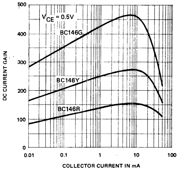
DC CURRENT GAIN VERSUS COLLECTOR CURRENT
