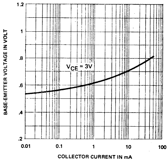
BASE-EMITTER VOLTAGE VERSUS COLLECTOR CURRENT
