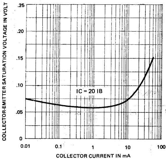
COLLECTOR-EMITTER SATURATION VOLTAGE VERSUS COLLECTOR CURRENT
