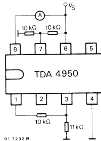
Figure 5 Test circuit 3
