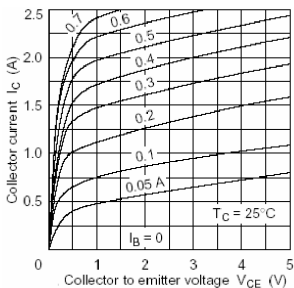
Fig.3 Static Characteristic
