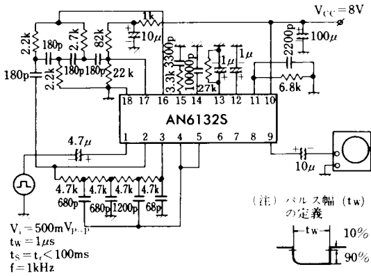
Test Circuit 3 ( t_w )
