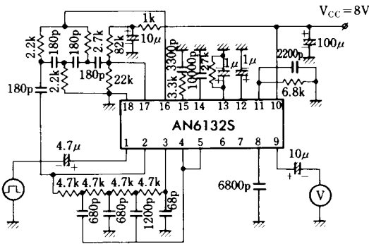
Test Circuit 5 ( V_{nr} )
