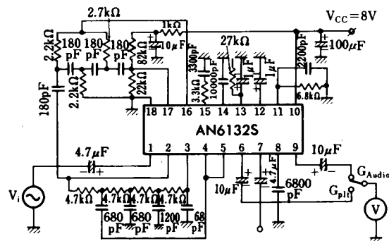
Test Circuit 1 (G A , G PI )
