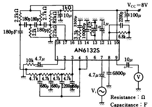
Test Circuit 2 (G PC )
