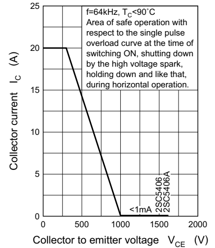
Area of safe operation, horizontal operation ASO
