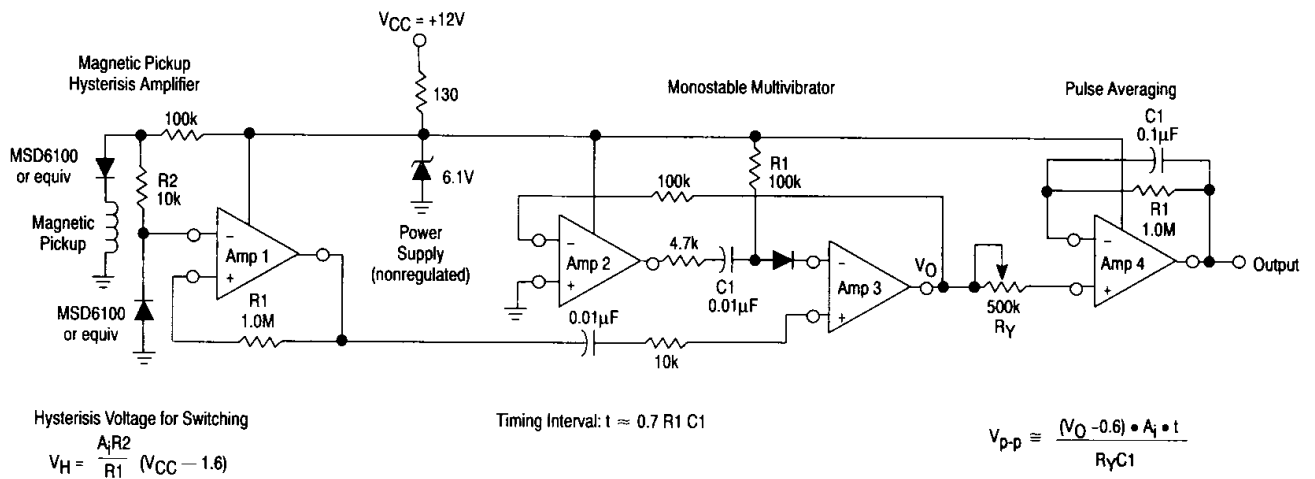
Figure 16. Tachometer Circuit
