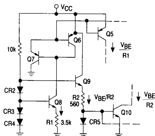
Figure 11. Biasing Circuitry
