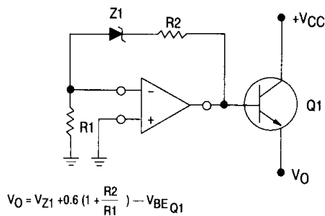
Figure 17. Voltage Regulator
