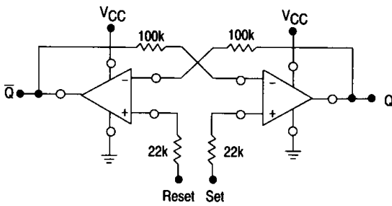
Figure 21. R-S Flip-Flop
