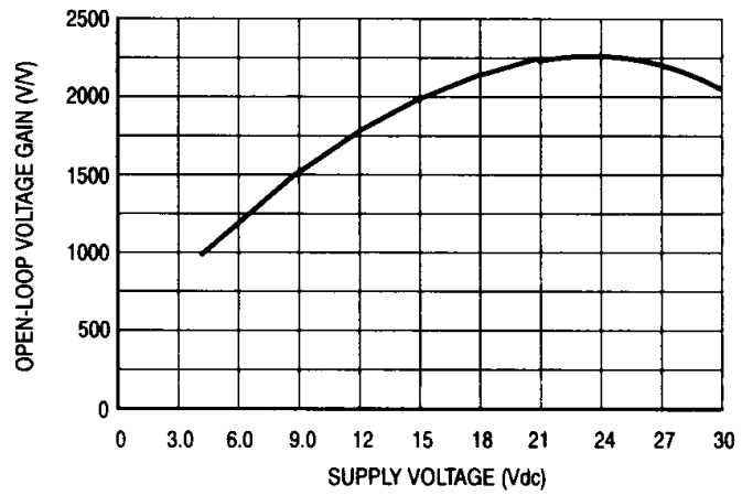
Figure 2. Open-Loop Voltage Gain versus Supply Voltage
