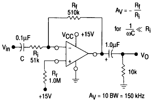
Figure 12. Inverting Amplifier
