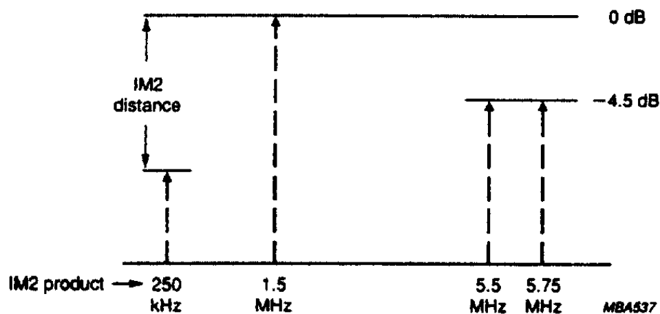
Fig.3 IM2 product.
