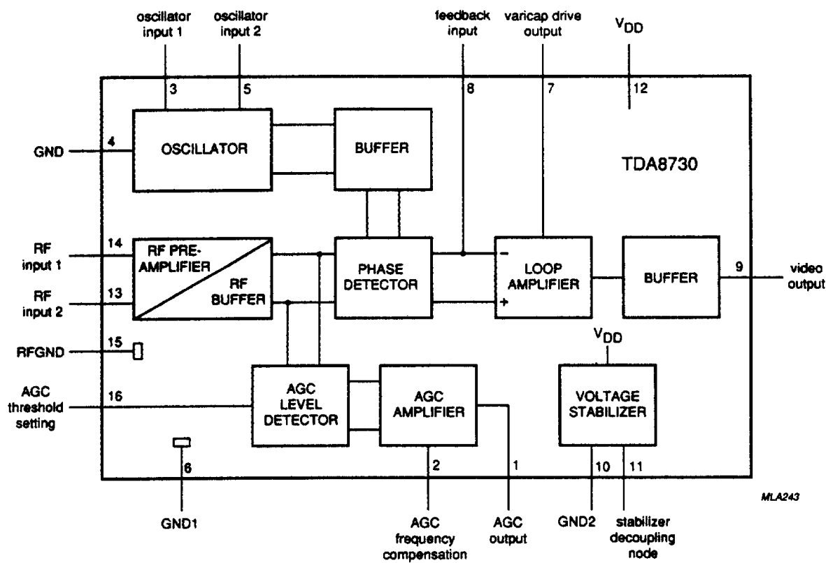
Fig.2 Block diagram.
