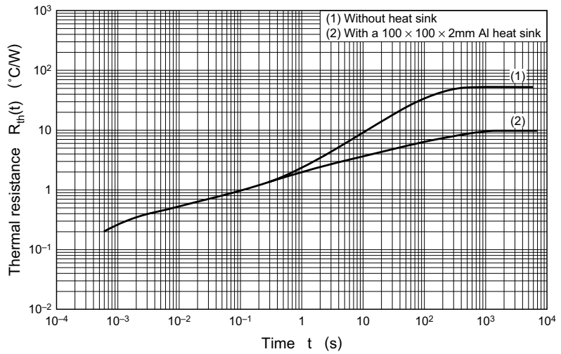
R_{th(t)} - t
